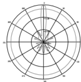
Vertical Pattern
