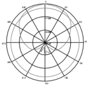
Horizontal Pattern
